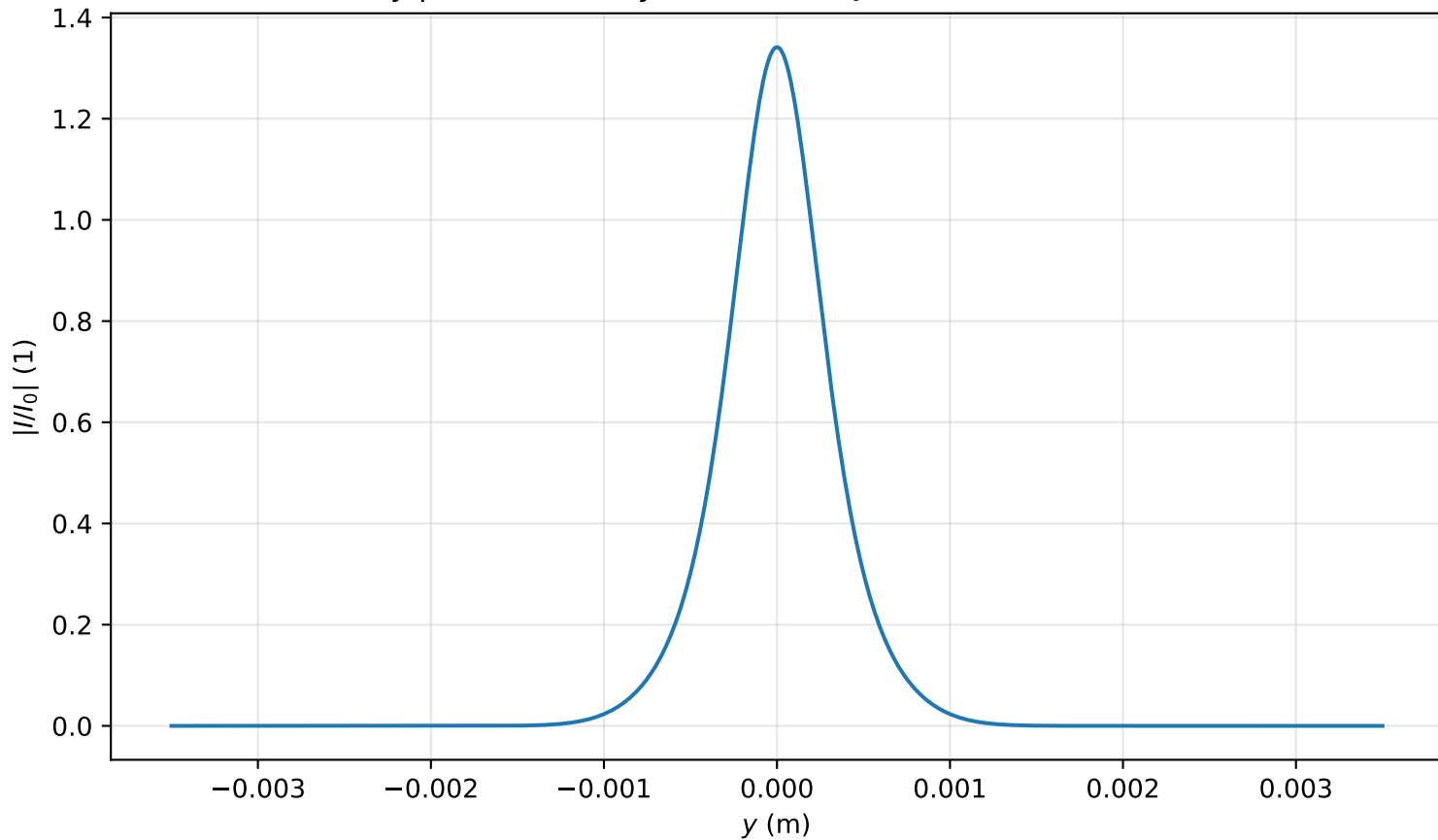
Intensity profile I(x=0, y, z=0.876)/I_0 , P_{in}=0.9P_{cr} , artificial time
